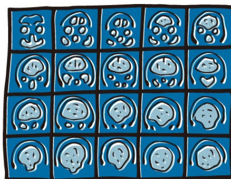
BRAIN SCAN
